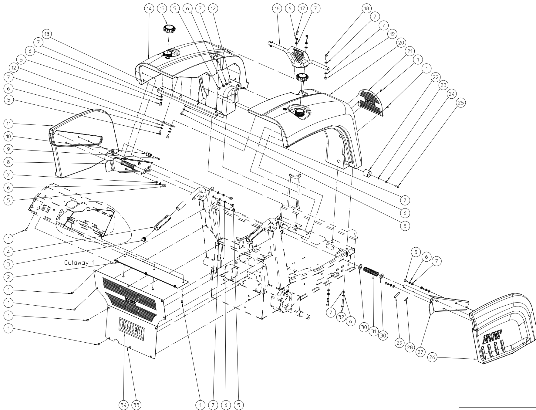
ELIET SNOWBOB -- SIDE COVER
